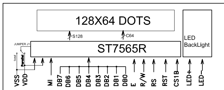
Driver Diagram
